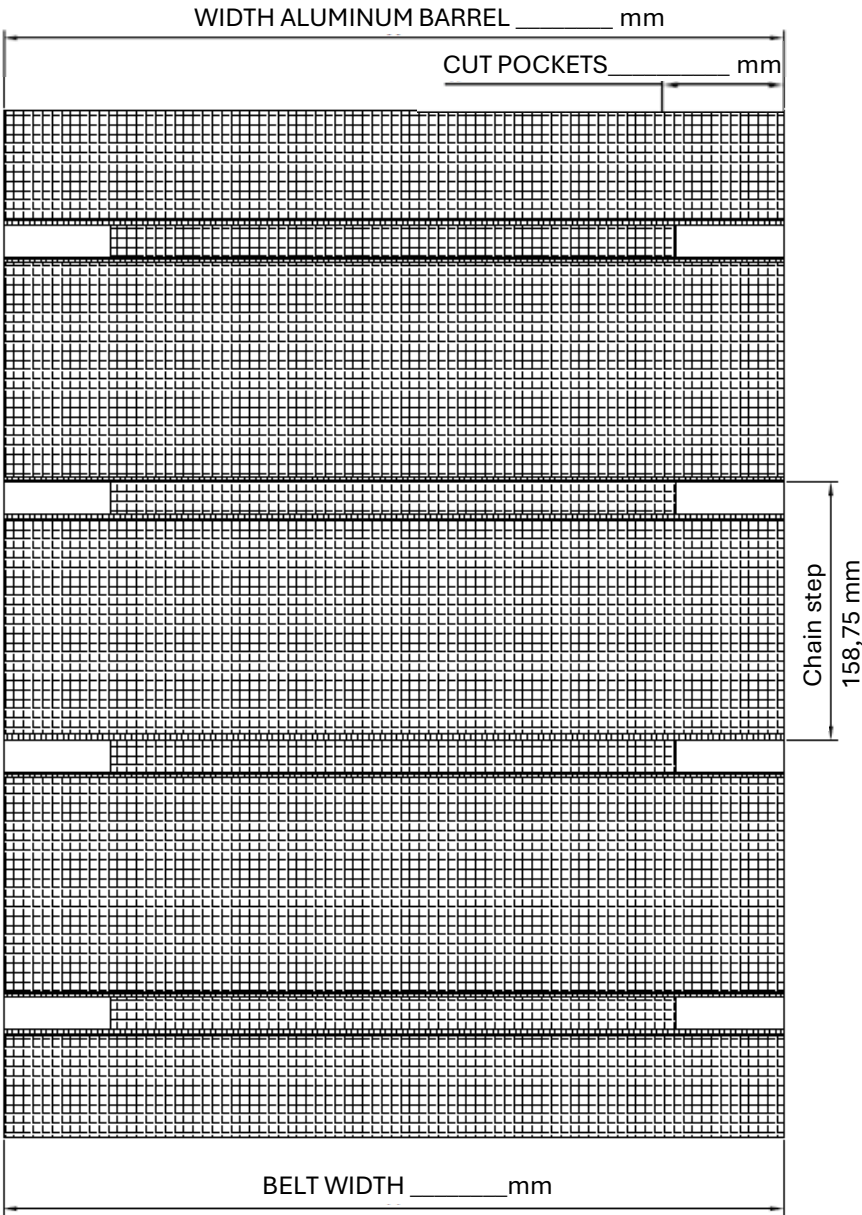
Section of aluminium barrel
