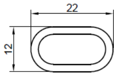
Section of aluminium barrel
