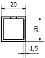
Section stainless steel
