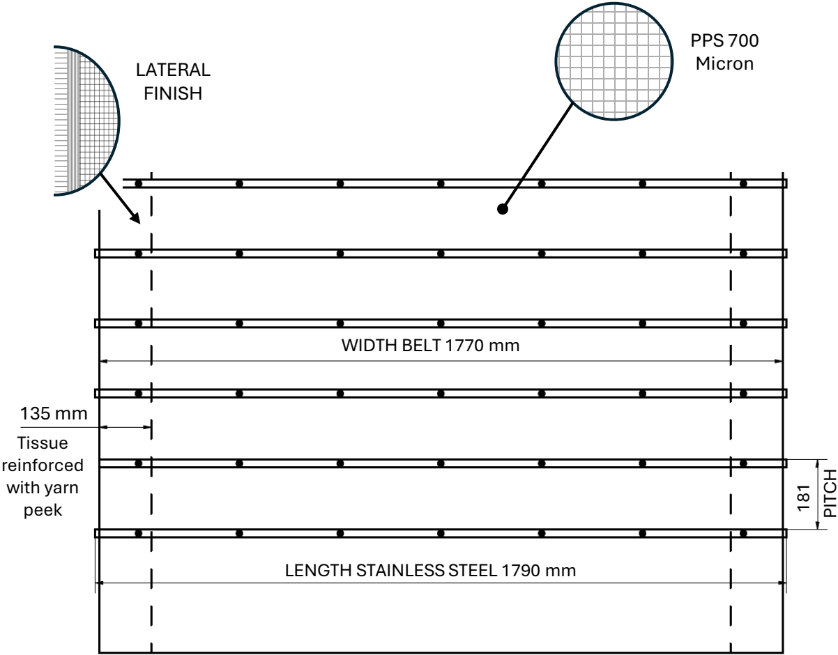
Section stainless steel
